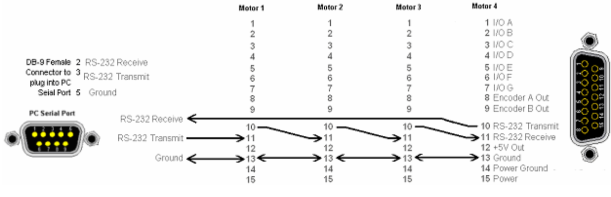
Serial Day Chain using the DB-15 connector
